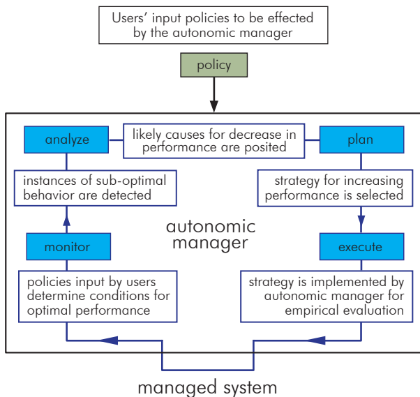
Figure: Schematic of a generalized autonomic manager. The MAPE loop is the iterative process by which user-defined policies are implemented to deal with constantly changing computing resources.
