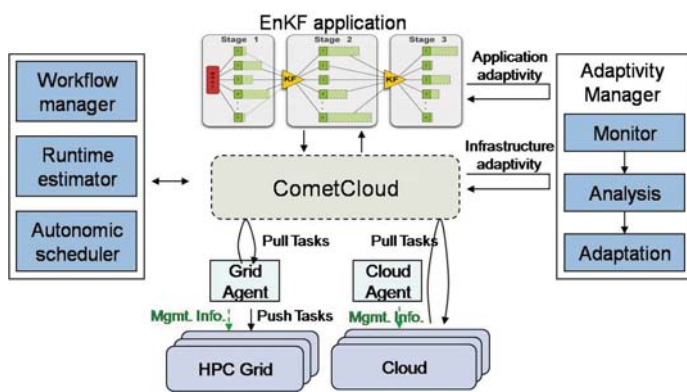
Figure: The MapReduce/CometCloud infrastructure: autonomic managers can adapt to changing resources and changing demands of applications. The Ensemble Kalman Filter (EnKF) application manages the multi-threaded workers that take advantage of multi-processor nodes.
