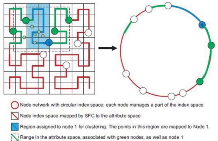
Figure: Overlay-based implementation of decentralized clustering technique
