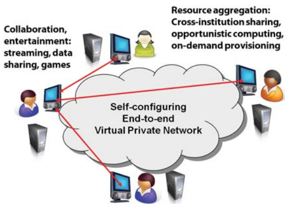
Figure: SocialVPN provides self-configuring virtual networks for collaboration.
