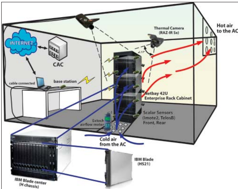
Figure: A schematic of the infrastructure for studying sensor-driven thermal management in data centers planned at Rutgers University. Autonomic redistribution of workload based on temperature profiles could decrease costs and improve performance in data centers used in a wide range of industries, from banking to utility services.
