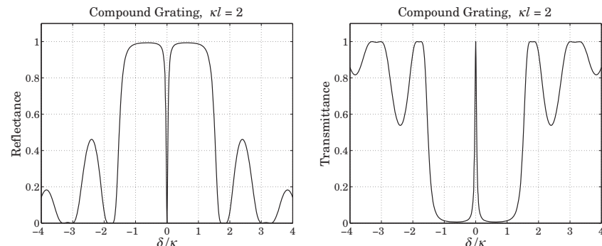
Fig. 12.5.4 Quarter-wave phase-shifted fiber Bragg grating.
