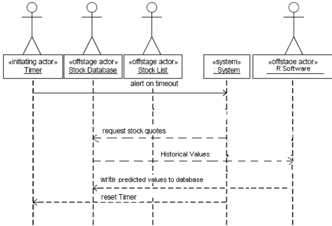
Figure 10: Use case diagram generating stock values and storing in database
