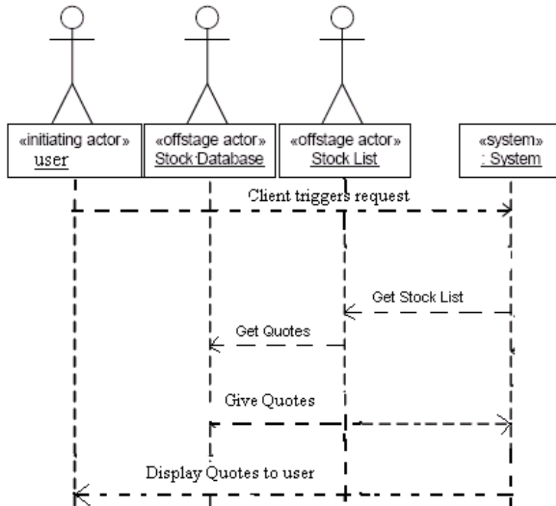
Figure 9: Use case diagram for displaying stock quotes at the client.
